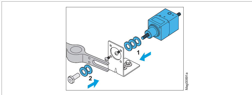
Fig. 73: Mount magnet, washers, and union nut (locked when de-energised.)
