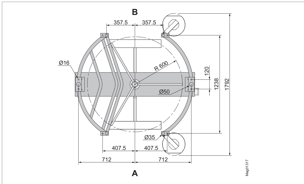
Fig. 8: Dimensions (size in mm) – MPT-333 (3x120°) with option “KHSB” View from below, Version “entrance side left” shown here, Illumination, twilight switch, and mounting pillars optional A Zone not controlled (ZNC) B Zone controlled (ZC)
