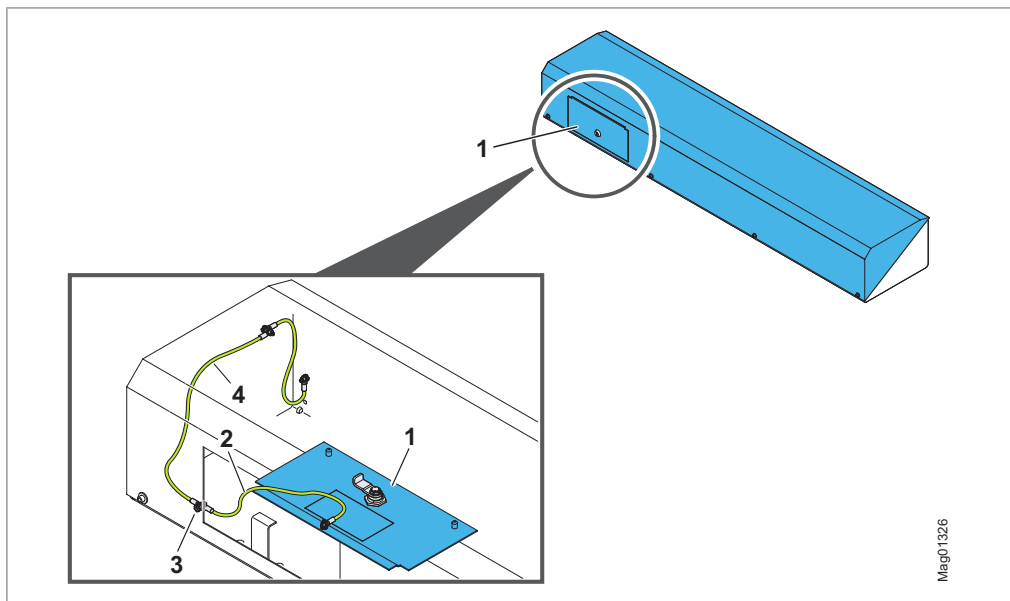
Fig. 59: Disconnect the protective earth conductor from the service door and cover
