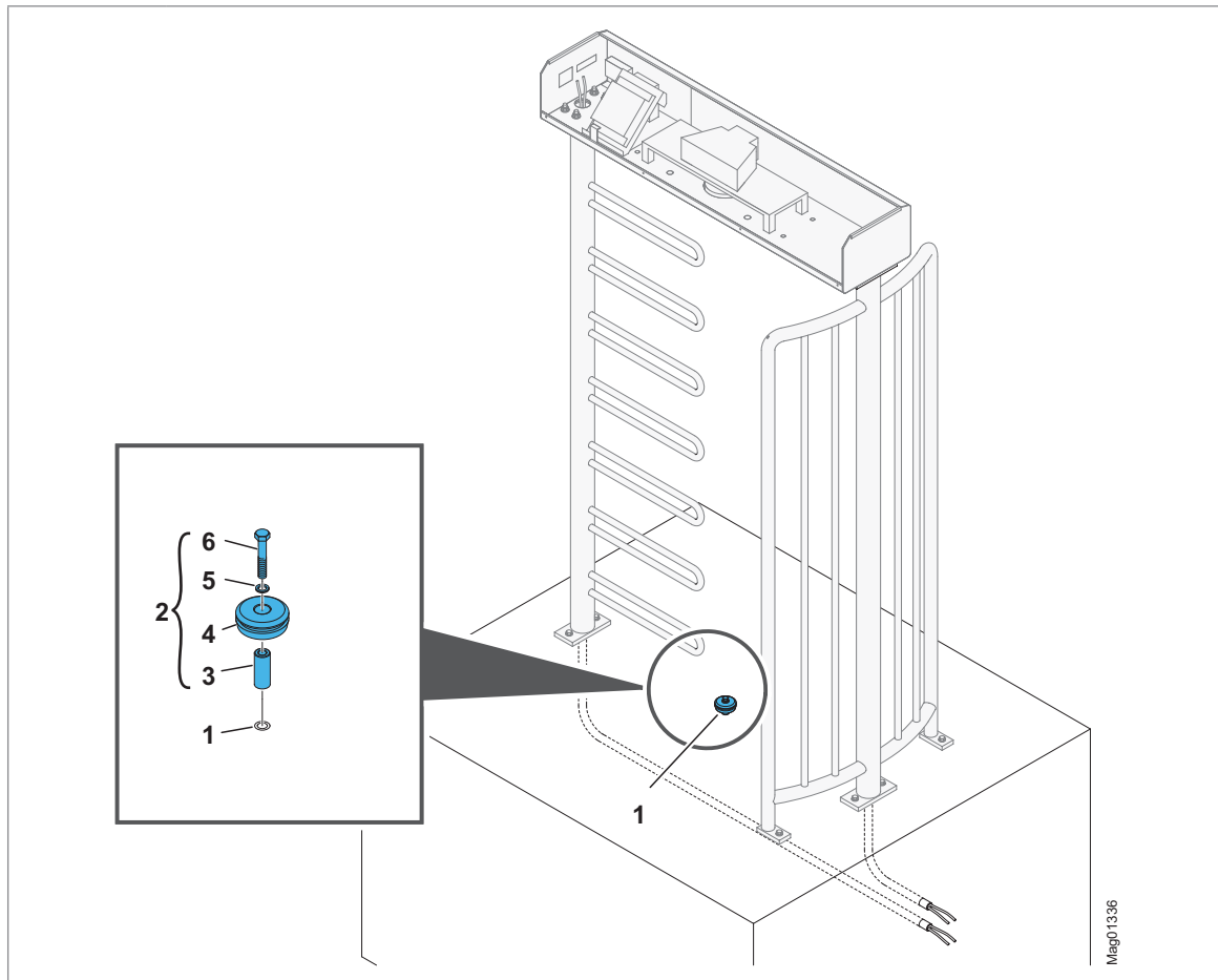
Fig. 43: Mounting the floor bearing – MPT-333 (4x90°)
