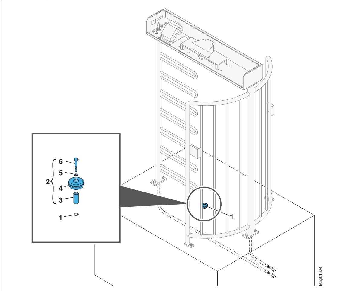
Fig. 31: Mounting the floor bearing – MPT-333 (3x120°)
