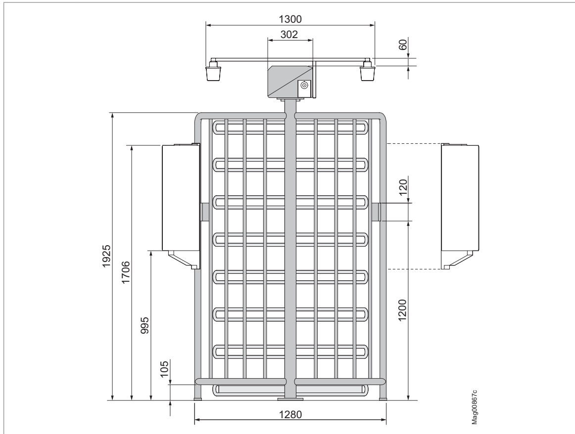
Fig. 4: Dimensions (size in mm) – MPT-333 (3x120°) Side view, Illumination, twilight switch, and mounting pillars optional, mounting height of mounting pillar for version by Magnetic
