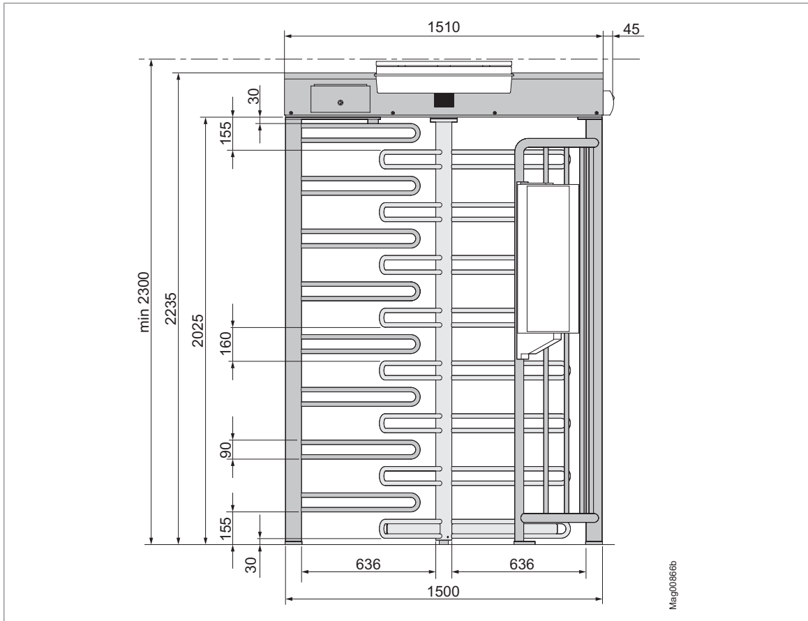
Fig. 3: Dimensions (size in mm) – MPT-333 (3x120°) View from zone controlled (ZC), Version “entrance side left” shown here Illumination, twilight switch, GED, and mounting pillars optional Required height min. 2300 mm to open the cover.
