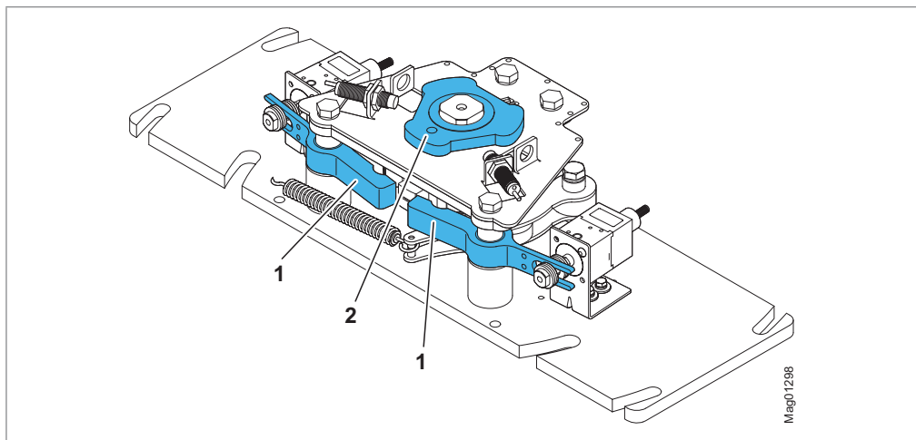
Fig. 33: Locking unit for centre pillar – MPT-3x3 (3x120°)
