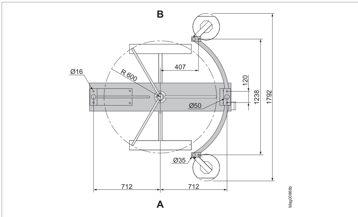
Fig. 5: Dimensions (size in mm) – MPT-333 (3x120°) View from below, Version “entrance side left” shown here, Illumination, twilight switch, and mounting pillars optional A Zone not controlled (ZNC) B Zone controlled (ZC)
