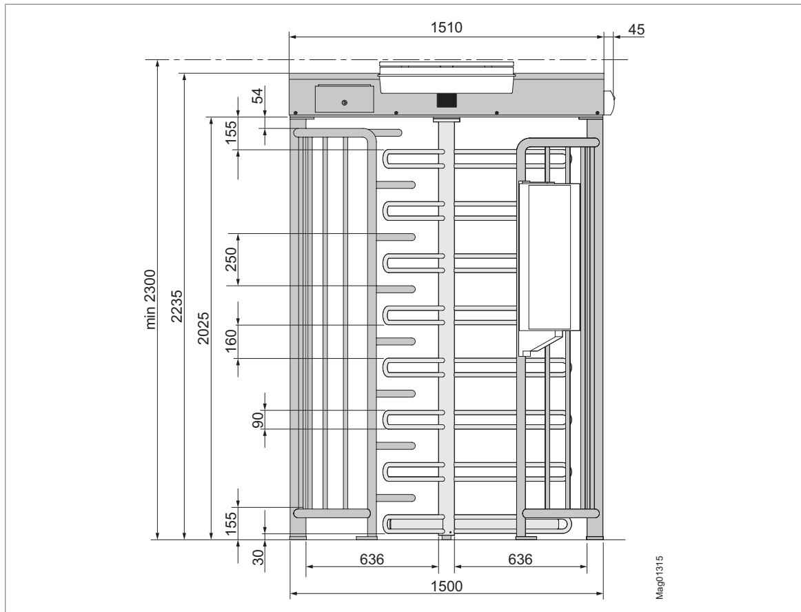
Fig. 6: Dimensions (size in mm) – MPT-333 (3x120°) with option “KHSB” View from zone controlled (ZC), Version “entrance side left” shown here Illumination, twilight switch, GED, and mounting pillars optional Required height min. 2300 mm to open the cover.
