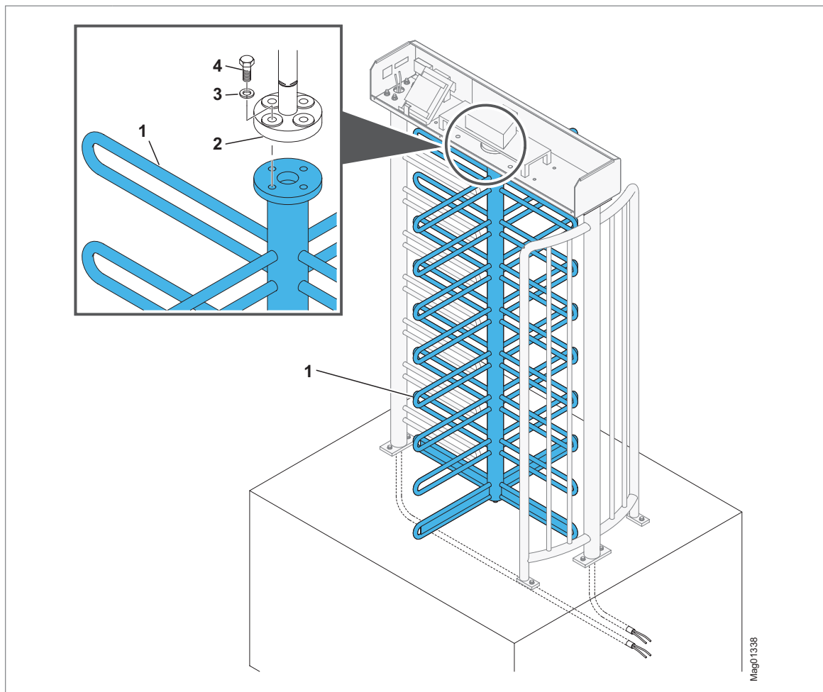
Fig. 47: Mounting the centre pillar on locking flange – MPT-333 (4x90°)
