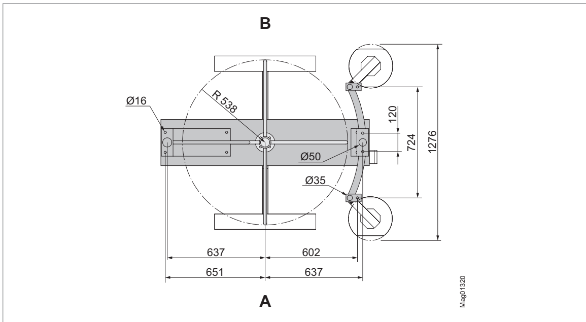
Fig. 11: Dimensions (size in mm) – MPT-333 (4x90°) View from below, Version “entrance side left” shown here, Illumination, twilight switch, and mounting pillars optional
