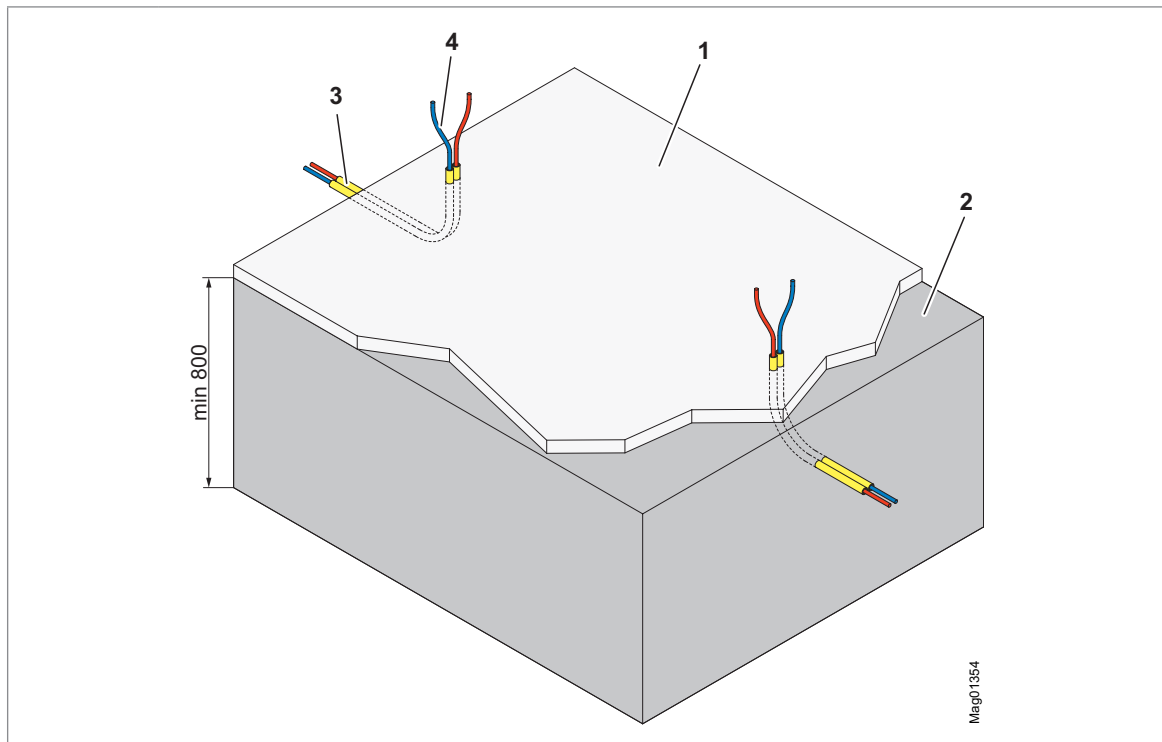
Fig. 20: Example of foundation design with empty tubes (size in mm)
