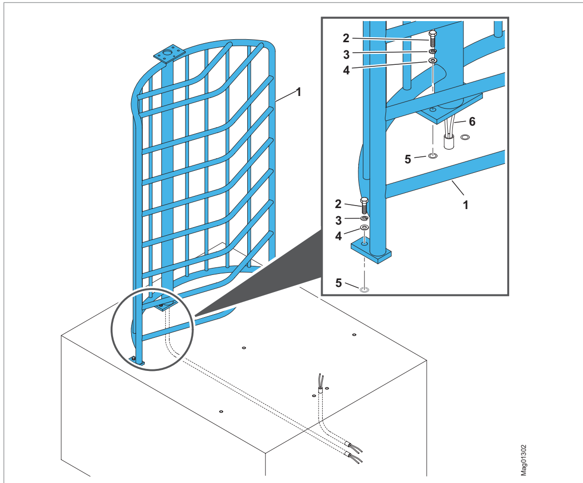
Fig. 26: Mounting the cage half with blocking bracket (option "KHSB")
