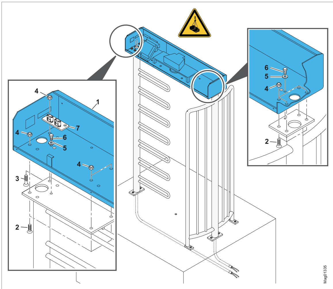
Fig. 42: Placing, earthing, and mounting the support beams – MPT-333 (4x90°)
