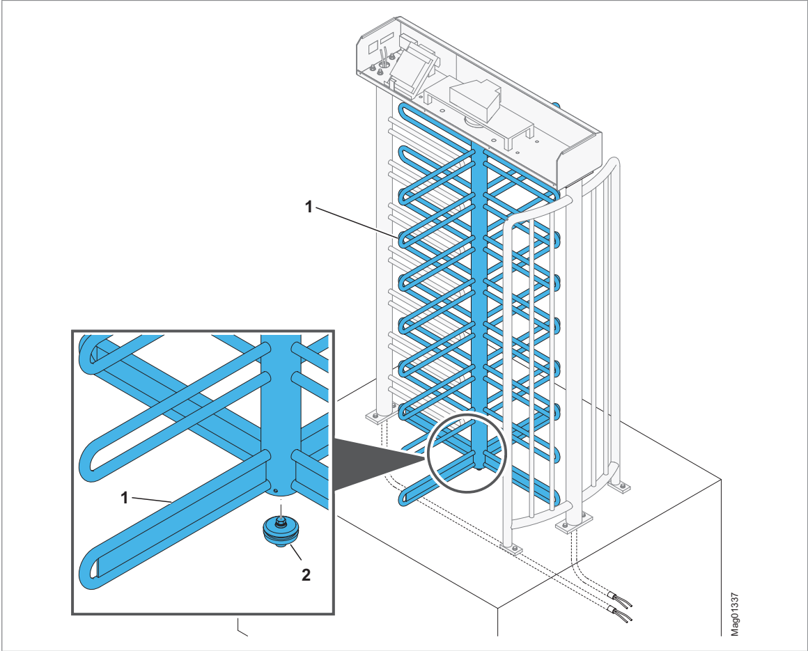
Fig. 44: Placing the centre pillar on floor bearing – MPT-333 (4x90°) 1 Centre pillar 2 Floor bearing
