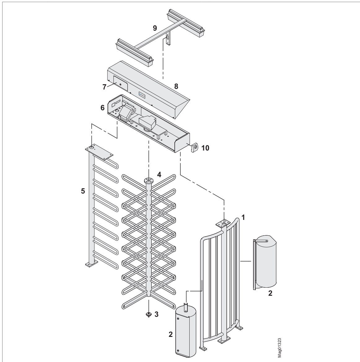
Fig. 14: Structure "Full height turnstile MPT-333 (4x90°)"
