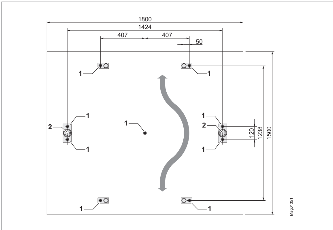
Fig. 22: Foundation and empty conduit plan MPT-333 (3x120°) with option “KHSB” for direct mounting on a foundation
