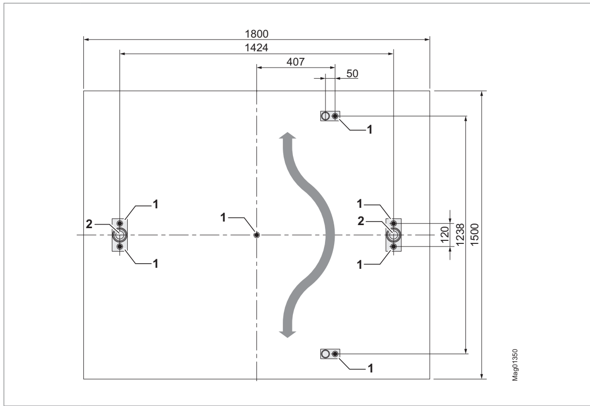
Fig. 21: Foundation and empty conduit plan MPT-333 (3x120°) for direct mounting on a foundation
