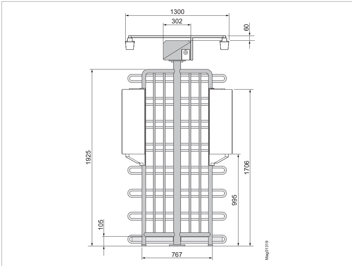
Fig. 10: Dimensions (in mm) – MPT-333 (4x90°) Side view, Illumination, twilight switch, and mounting pillar optional, Dimensions of mounting pillar for version by Magnetic
