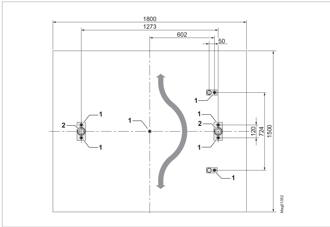
Fig. 23: Foundation and empty conduit plan MPT-333 (4x90°) for direct mounting on a foundation
