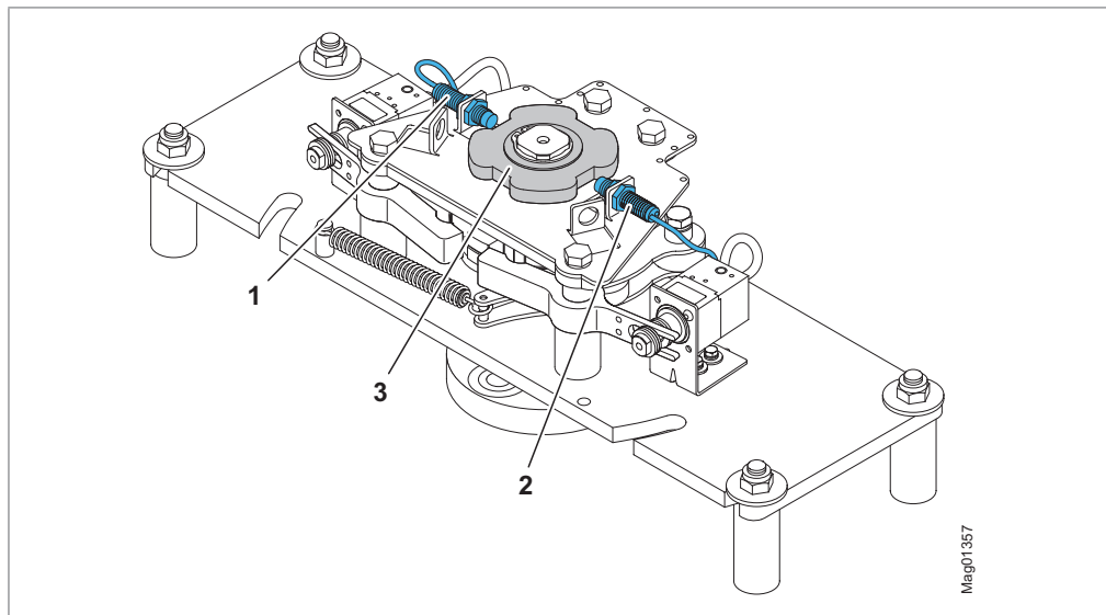
Fig. 66: Proximity sensors to detect the end position of the centre pillar, locking unit for MPT-3x3 (4x90°)
