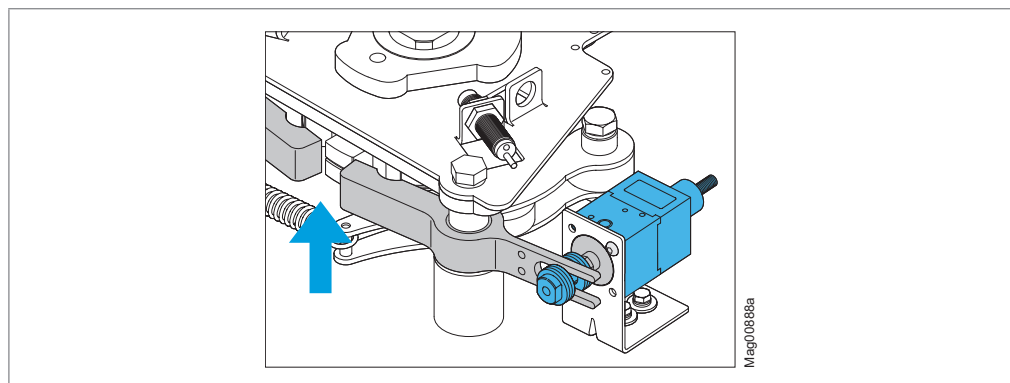
Fig. 70: Locking unit configuration “rotating freely when de-energised” (here locking unit for MPT-3x3 (3x120°) shown)
