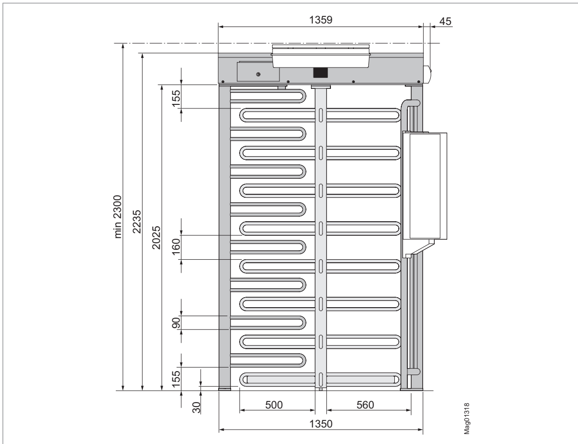
Fig. 9: Dimensions (size in mm) – MPT-333 (4x90°) View from zone controlled (ZC), Version “entrance side left” shown here Illumination, twilight switch, GED. and mounting pillars optional Required height min. 2300 mm to open the cover.
