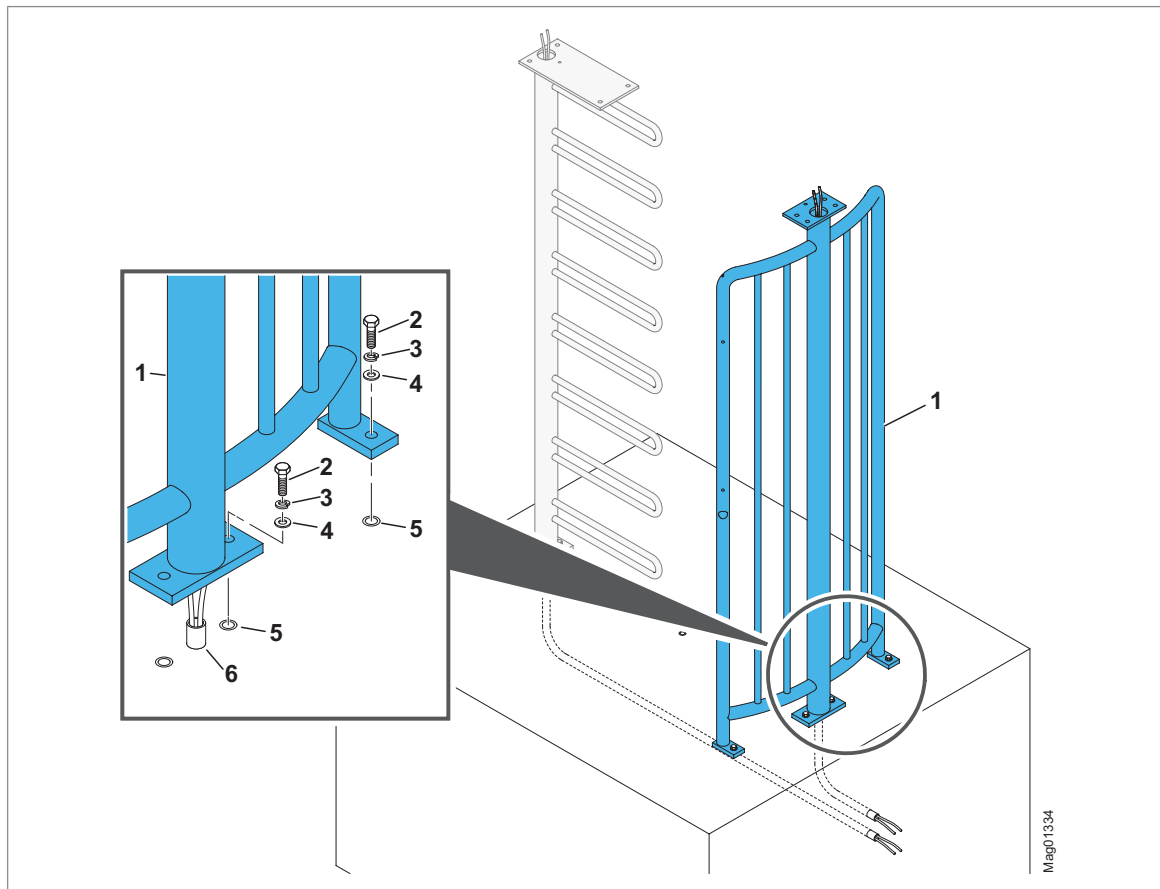
Fig. 39: Mounting the cage half – MPT-333 (4x90°)
