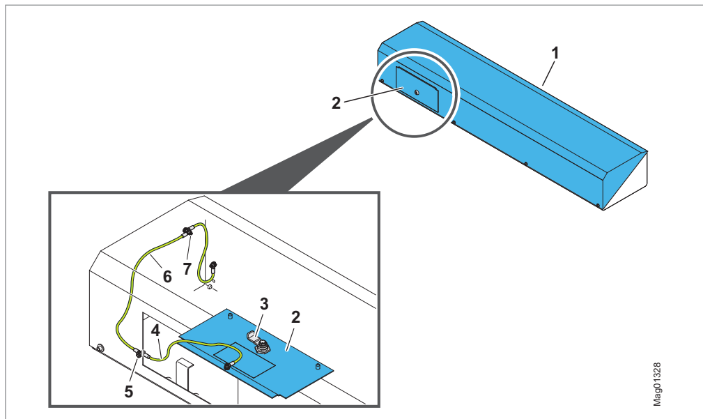
Fig. 37: Earthing of cover and service door (exemplary representation)
