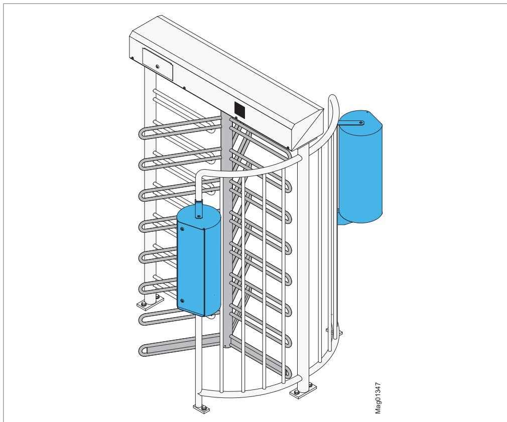
Fig. 50: Optional mounting pillars – example MPT-333 (3x120°)
