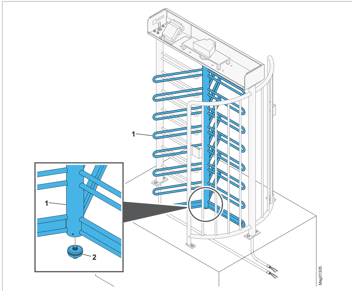
Fig. 32: Placing the centre pillar on floor bearing – MPT-333 (3x120°)
