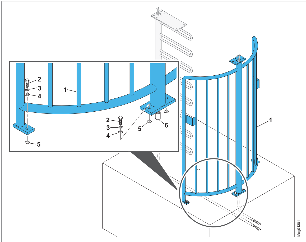
Fig. 27: Mounting the cage half – MPT-333 (3x120°)
