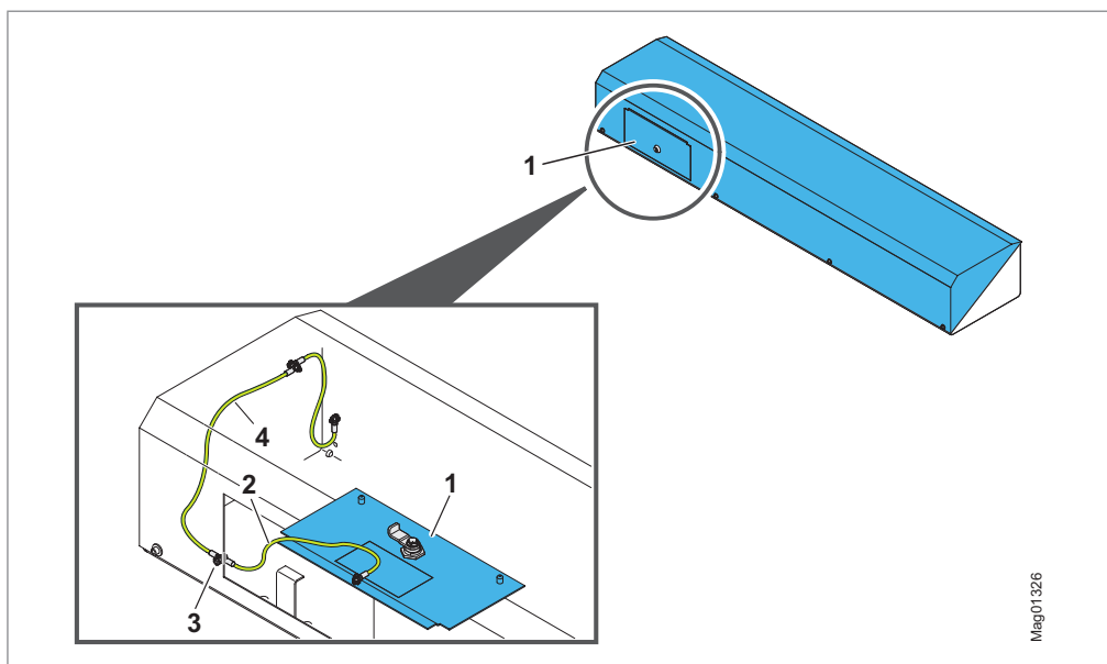
Fig. 40: Disconnect the protective earth conductor from the service door and cover
