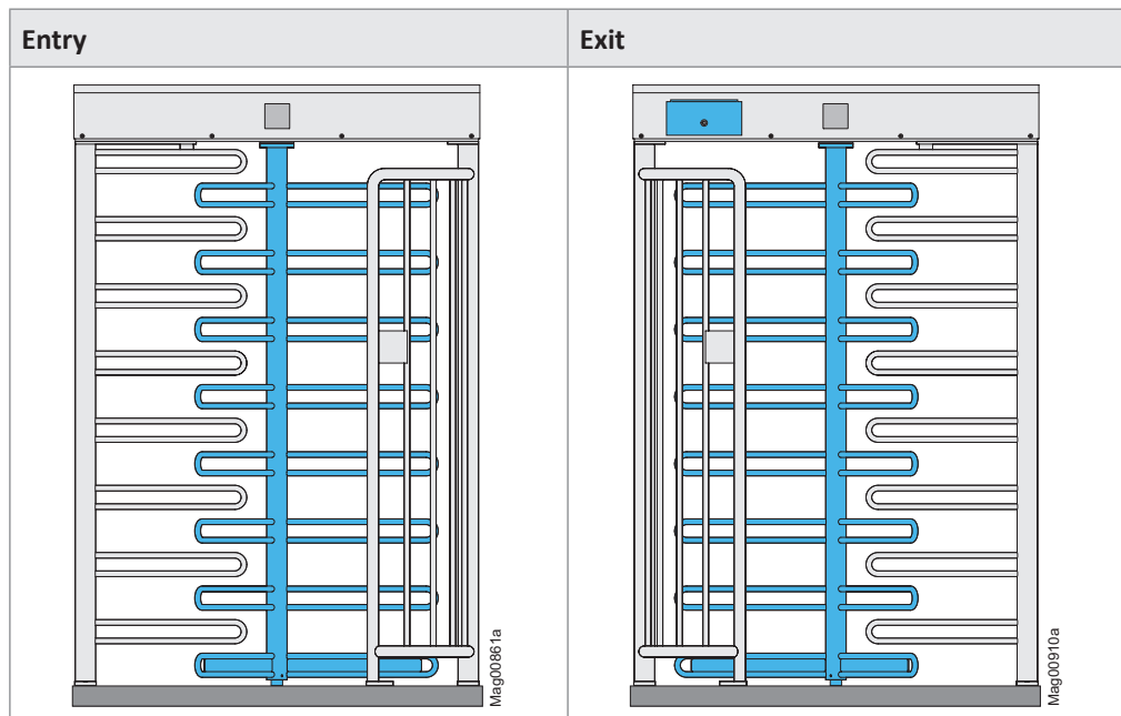
Fig. 15: Version “Entrance side right”, here MPT-x3x 3x120° – view from the zone not controlled (ZNC), the entry is to the right of the centre pillar
