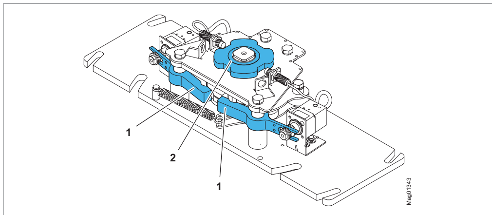
Fig. 45: Locking unit for centre pillar – MPT-3x3 (4x90°)
