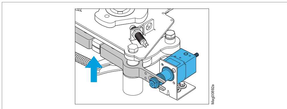
Fig. 74: Locking unit configuration “locked when de-energised” (locking unit for MPT-3x3 (3x120°) is shown here)
