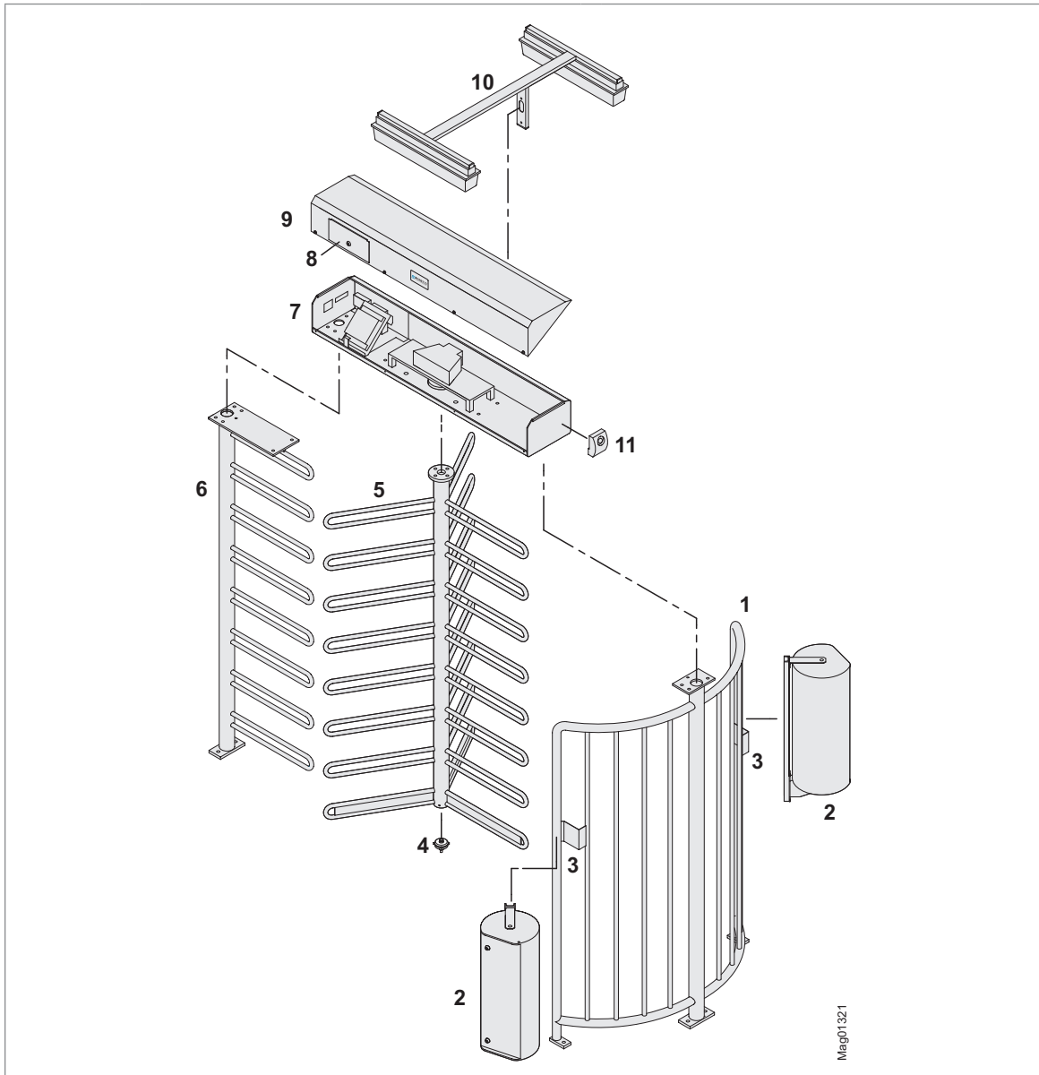
Fig. 12: Design "Full height turnstile MPT-333 (3x120°)"
