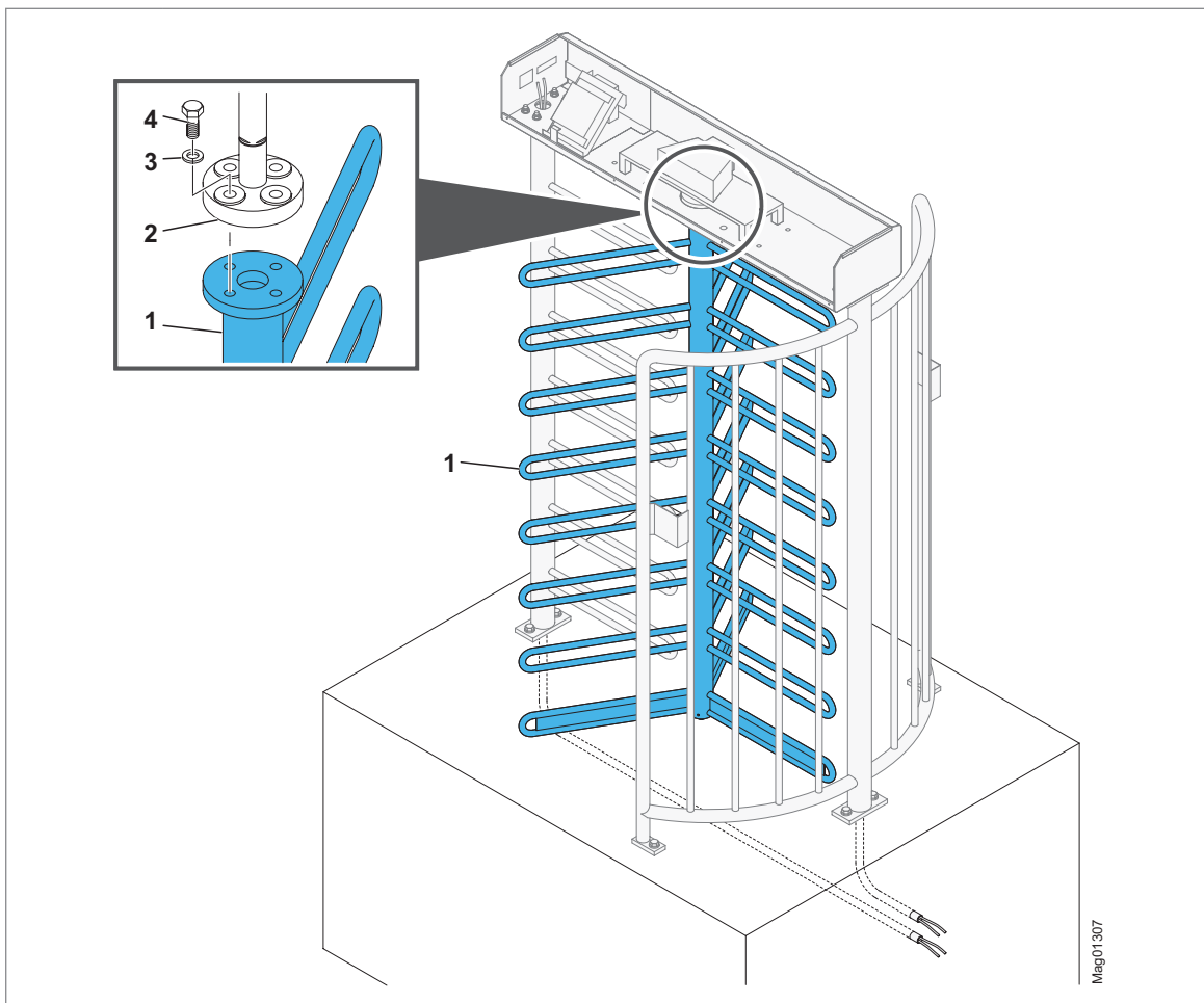
Fig. 35: Mounting the centre pillar on locking flange – MPT-333 (3x120°)
