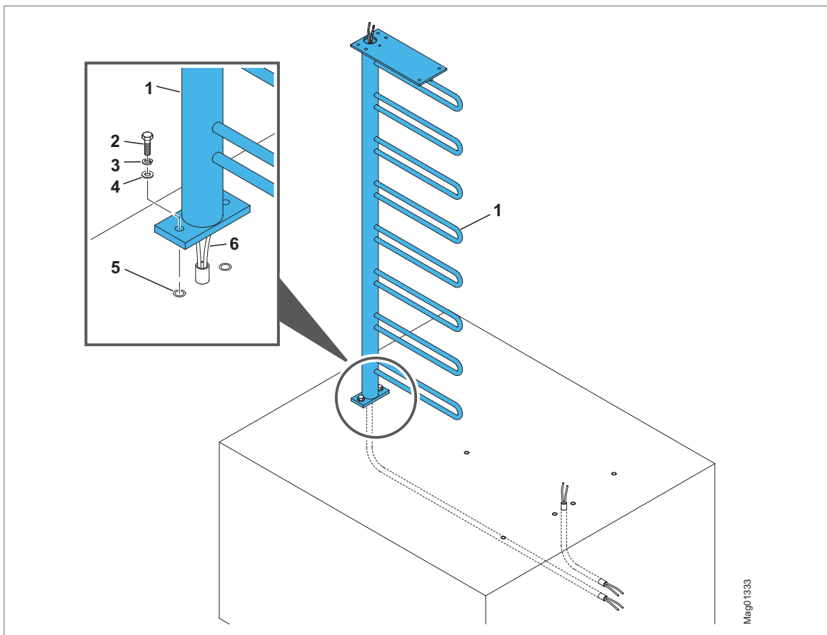
Fig. 38: Mounting the locking comb – MPT-333 (4x90°)
