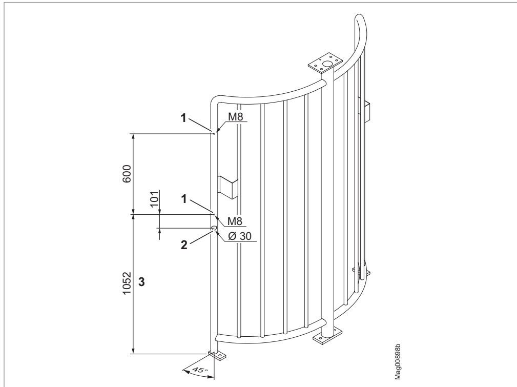
Fig. 51: Required holes for mounting pillar (all size in mm)
