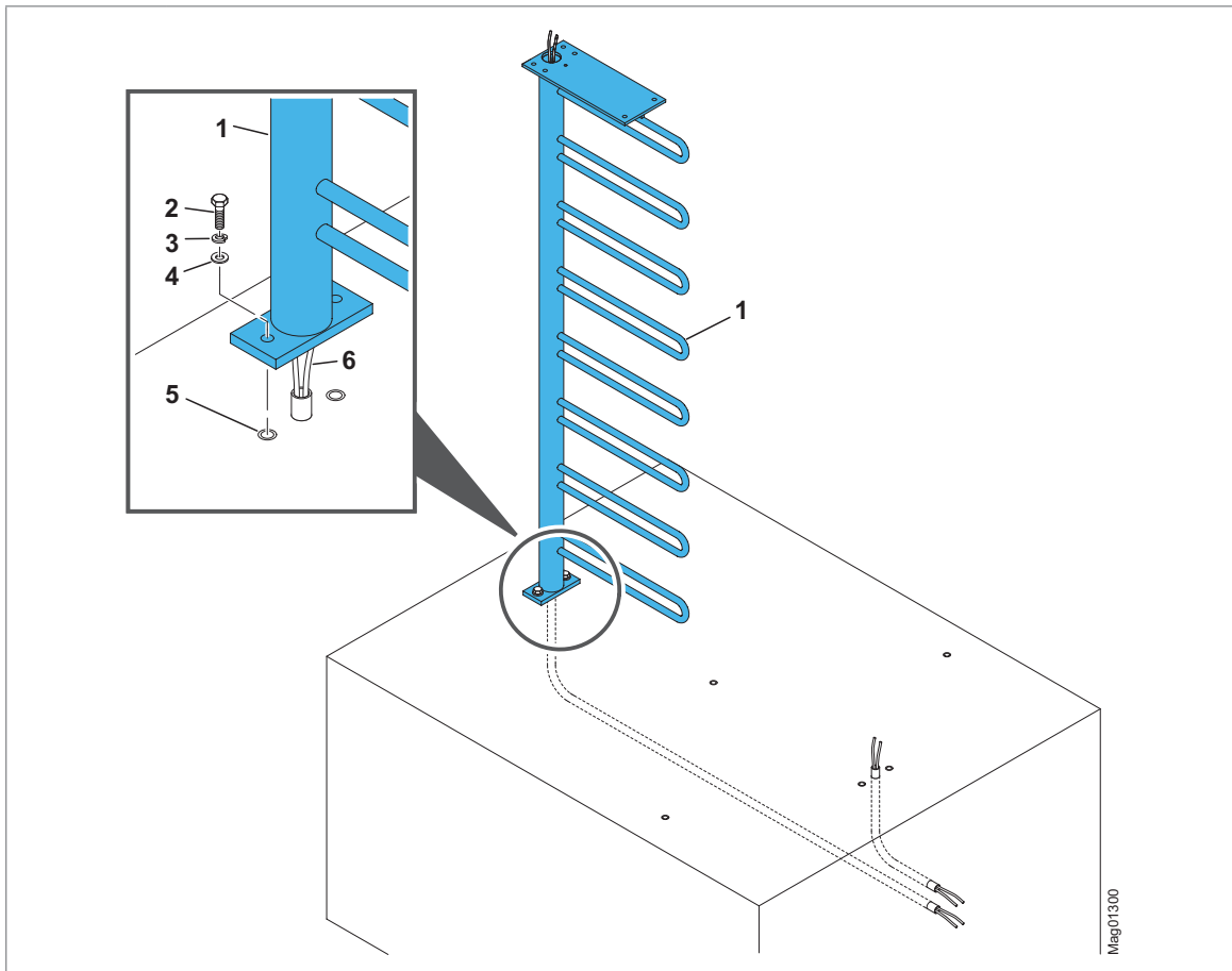
Fig. 25: Mounting the locking comb – MPT-333 (3x120°)
