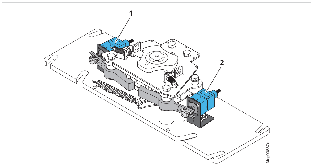
Fig. 69: Locking unit configuration “rotating freely when de-energised” – locking unit for MPT-3x3 (3x120°) shown here, designations and position of the magnets for locking unit MPT-3x3 (4x90°) are identical
