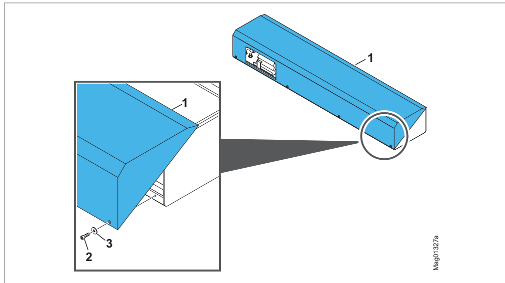
Fig. 41: Opening the cover
