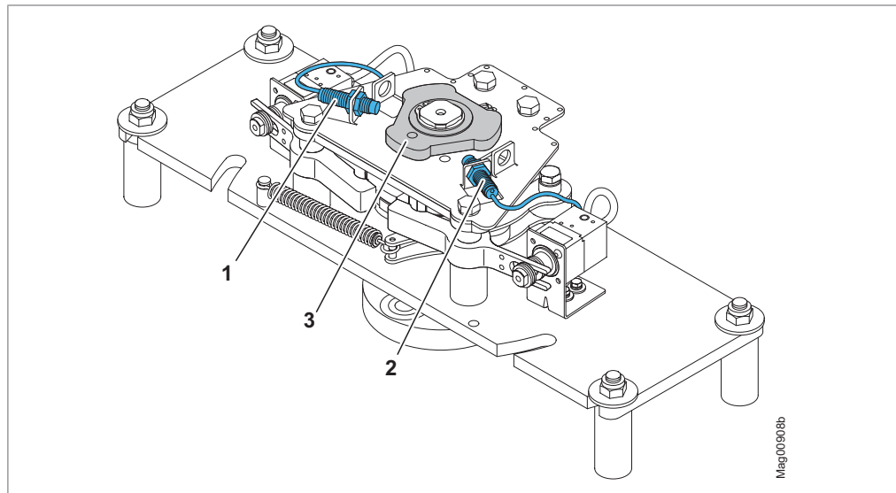
Fig. 65: Proximity sensors to detect the end position of the centre pillar, locking unit for MPT-3x3 (3x120°)
