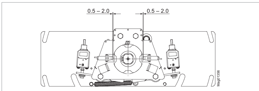
Fig. 68: Distance proximity sensor – switching cam for locking unit for MPT-3x3 (4x90°)
