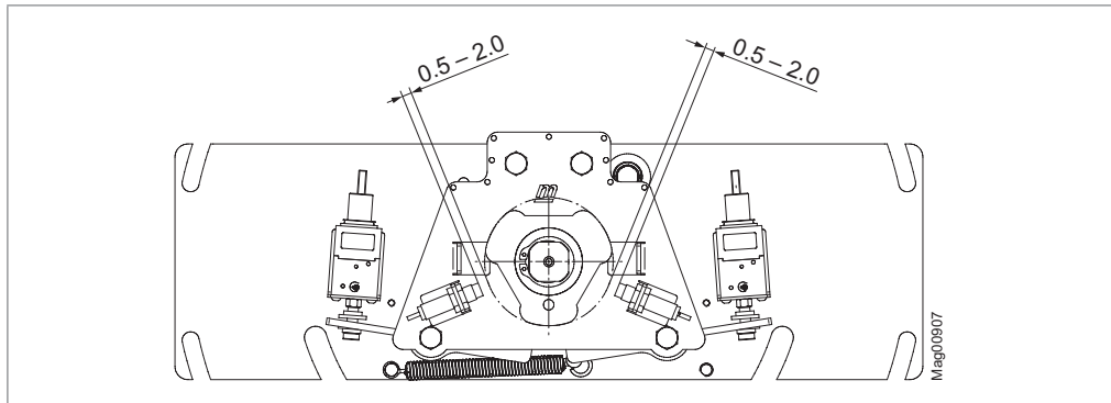
Fig. 67: Distance proximity sensor – switching cam for locking unit for MPT-3x3 (3x120°)
