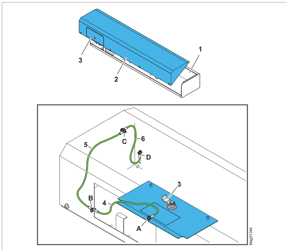
Fig. 1: Earthing support beam, cover, and service door (exemplary representation)
