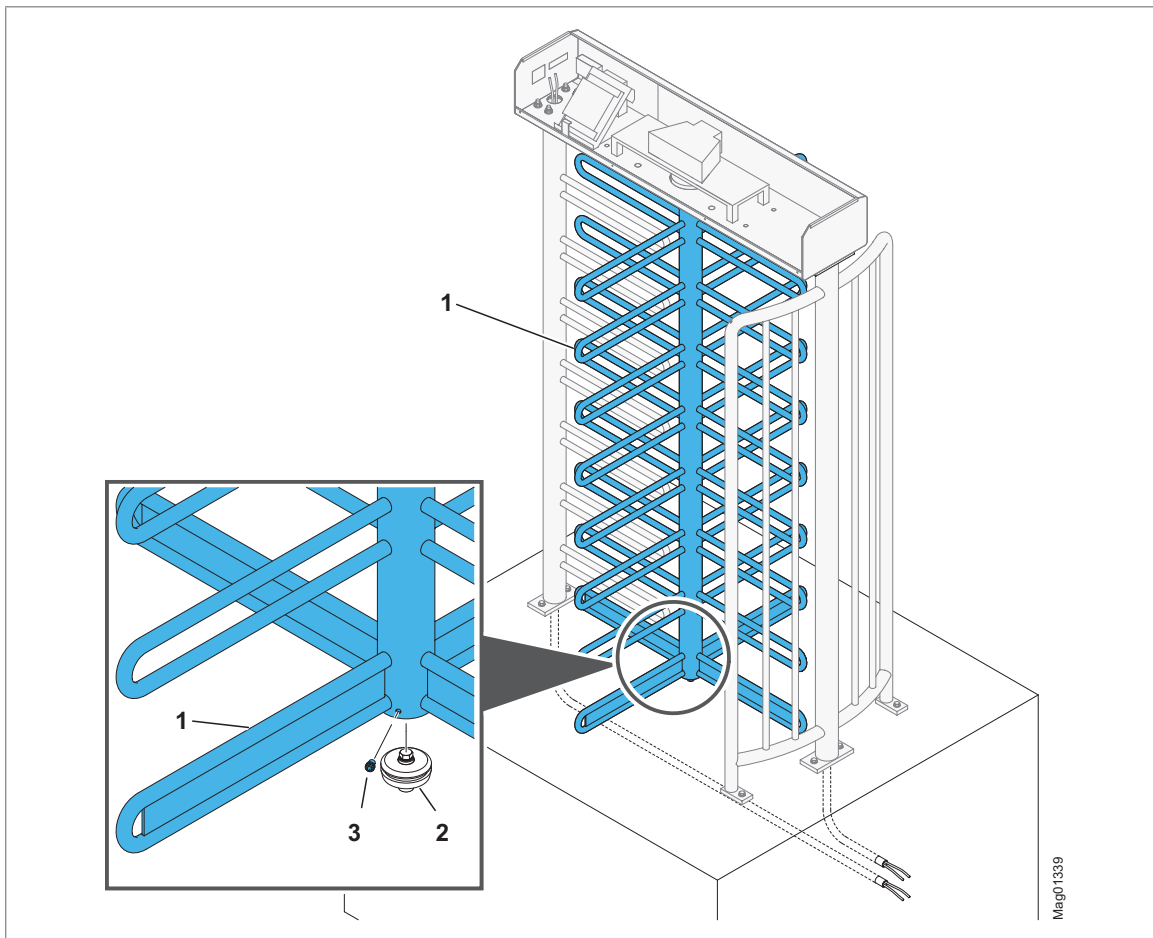
Fig. 48: Fixing the centre pillar to the floor bearing – MPT-333 (4x90°)
