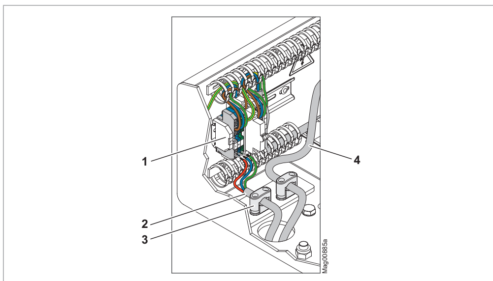
Fig. 63: Connecting the mains cable
