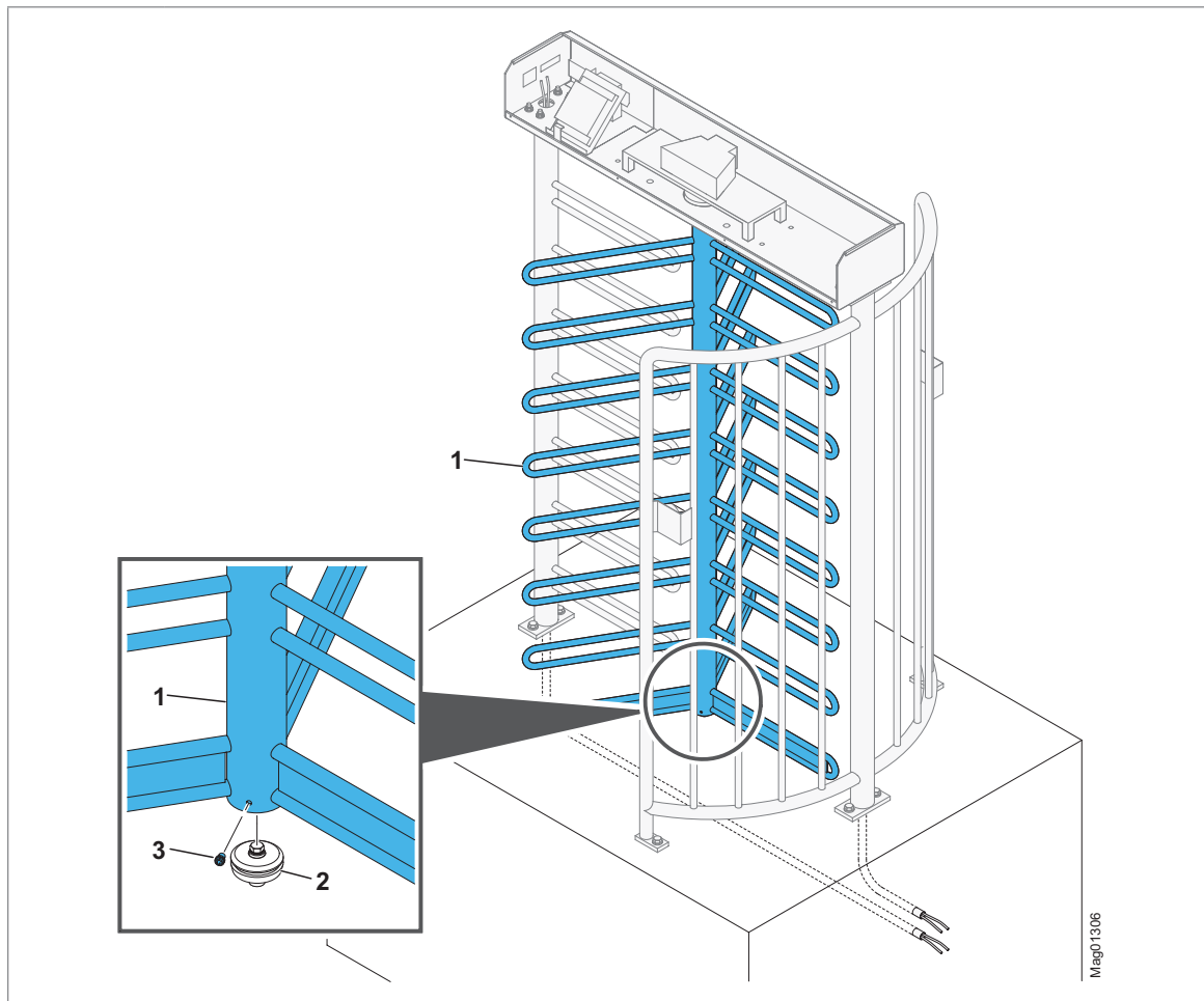
Fig. 36: Fixing the centre pillar to the floor bearing – MPT-333 (3x120°)
