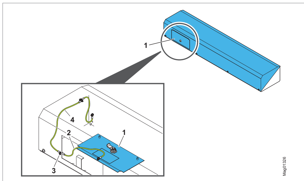
Fig. 28: Disconnect the protective earth conductor from the service door and cover (exemplary representation)
