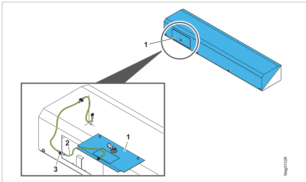
Fig. 61: Open the service door, grounding of the service door (exemplary representation)
