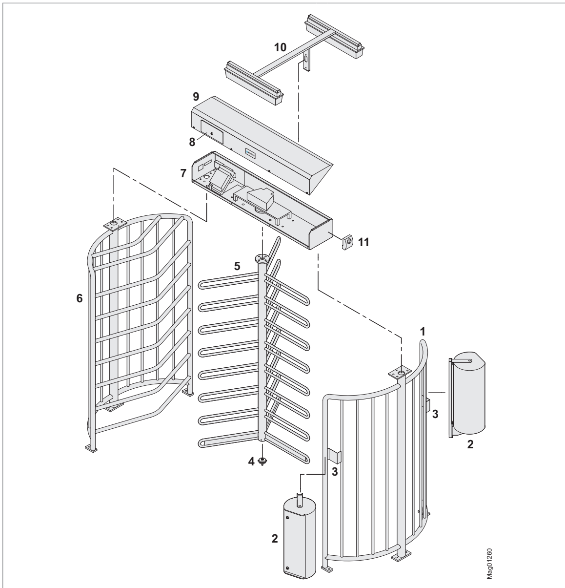
Fig. 13: Setup “Full height turnstile MPT-333 (3x120°)” with option “KHSB”
